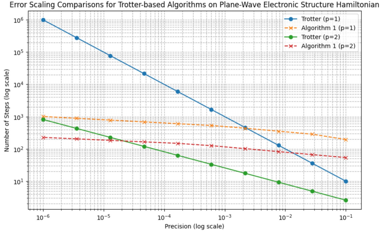
Figure 1: Comparison of total simulation steps required by the standard Trotter method and Algorithm 1 using well-conditioned extrapolation points, for different error tolerances and Trotter orders.
