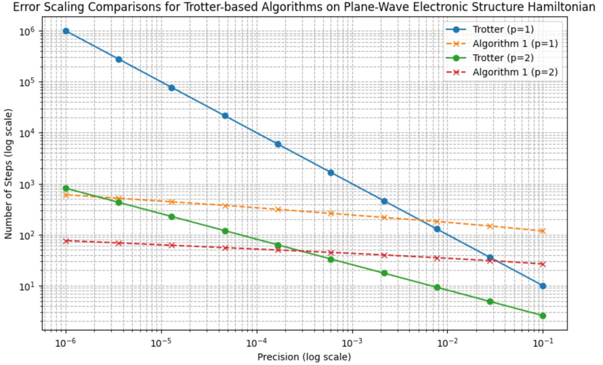
Figure 2: Comparison of total simulation steps required by the Trotter method and Algorithm 1 after brute-force optimization over extrapolation points, for different error tolerances and Trotter orders.
